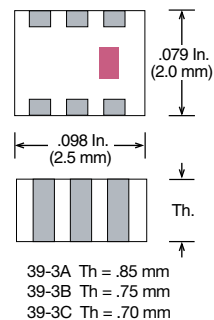
Case 39-3 (2520)
