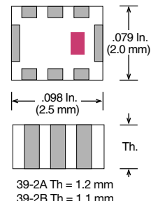
Case 39-2 (2520)
