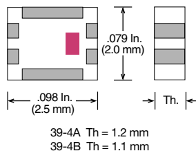
Case 39-4 (2520)
